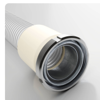
Combiflex Dairy Fitting Cone Sockets cast-on tube fitting with groove nut to DIN 11851 for Master-PUR Food hoses, food-safe EU 10/2011
