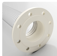
Combiflex Cast-on PU Fixed Flange Food fixed flange for all Master-PUR Food hose types, approved for direct food contact EU 10/2011, for counterflanges acc. to DIN 2632 / DIN 2633 / DIN 2673
